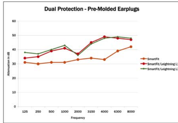
Graph 2. Dual Protection with Pre-Molded Earplugs
