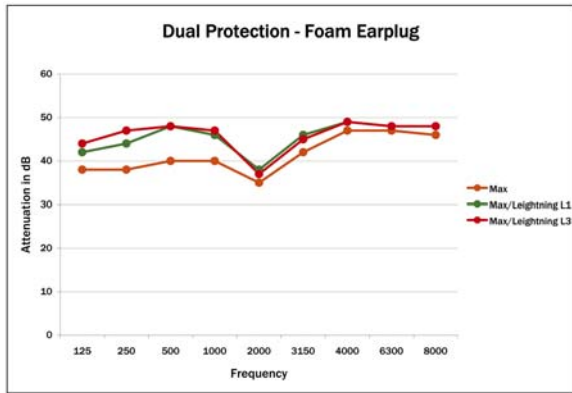
Graph 1. Dual Protection with Foam Earplugs
